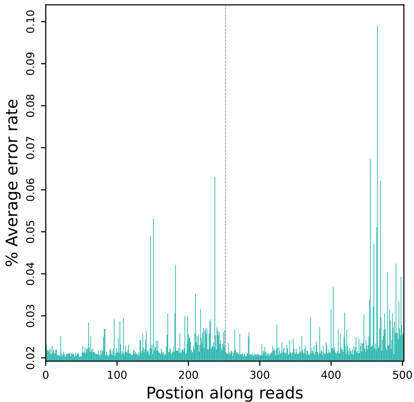
Error rate distribution along reads (R10611)
